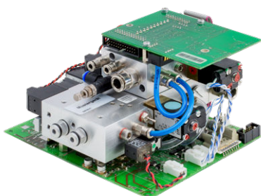
Digital Gas Mixer
